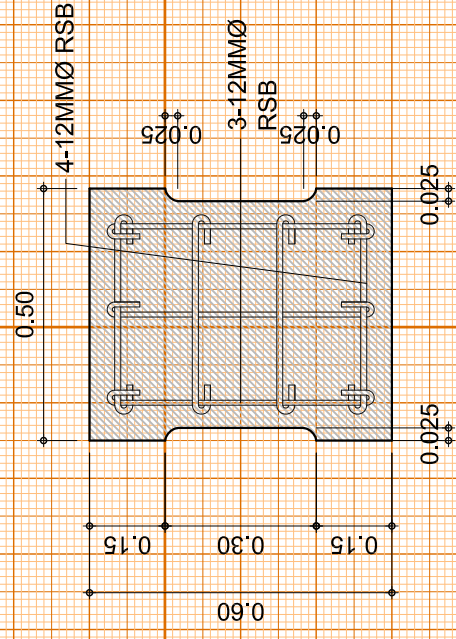
DETAIL OF DETACHABLE CONCRETE COVER
