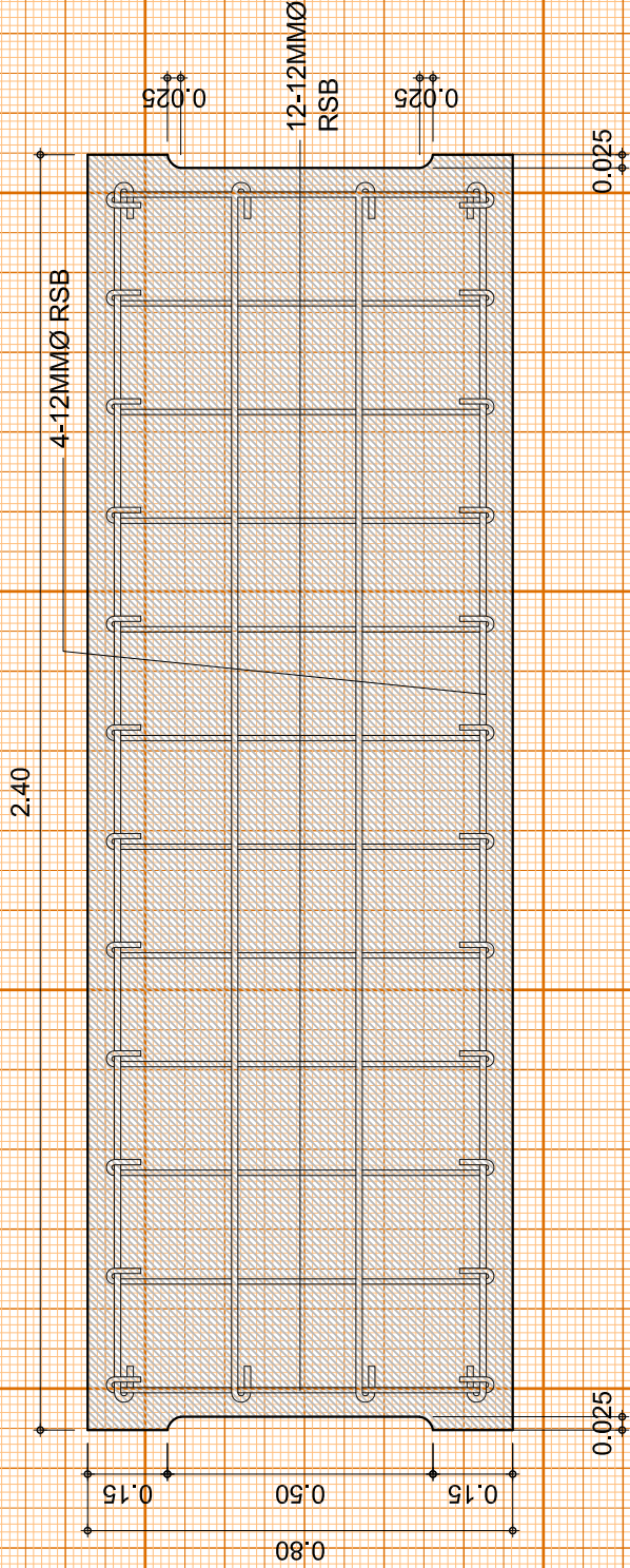
DETAIL OF FIXED CONCRETE COVER SCALE: 1:15 METERS
